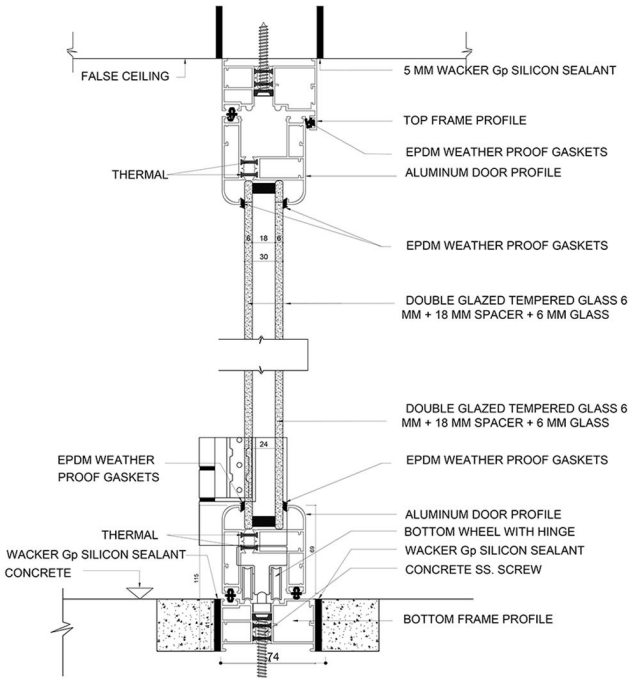
VERTICAL SECTION DETAILS
