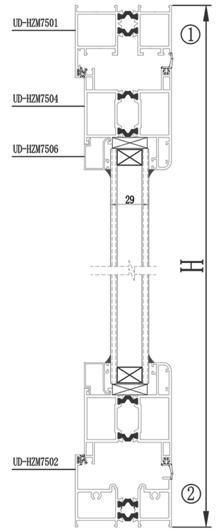
SECTION
