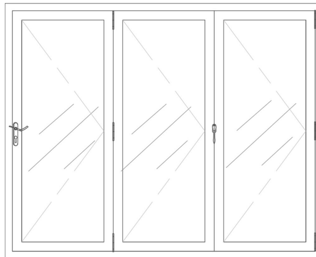
ELEVATION FROM INSIDE
